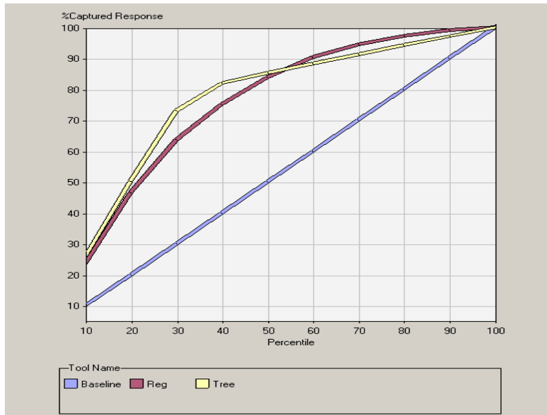
Figure 3. Lift Chart Comparing a Regression Model to a Decision Tree
